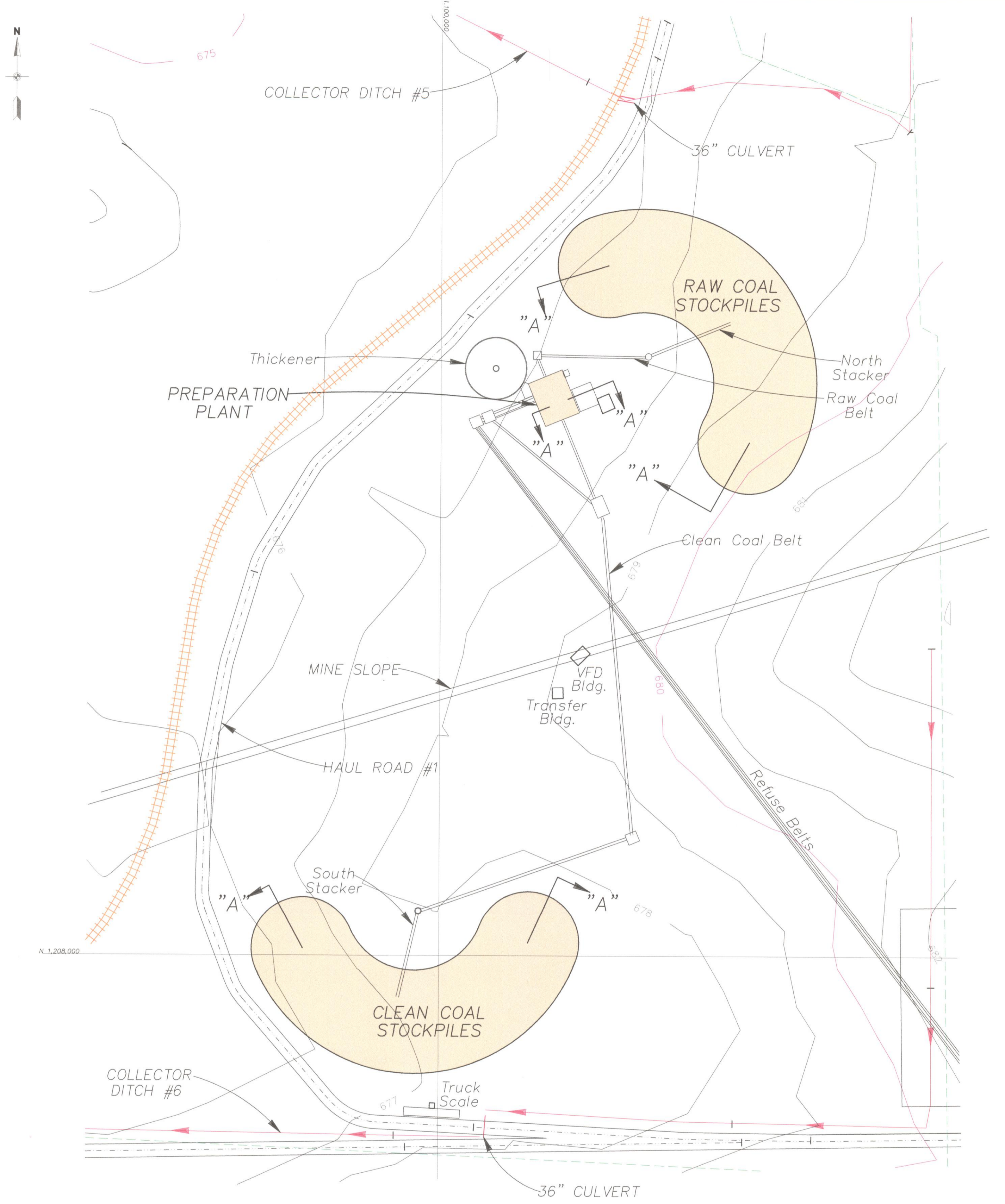
LOCATION MAP SCALE: 1" = 100'
