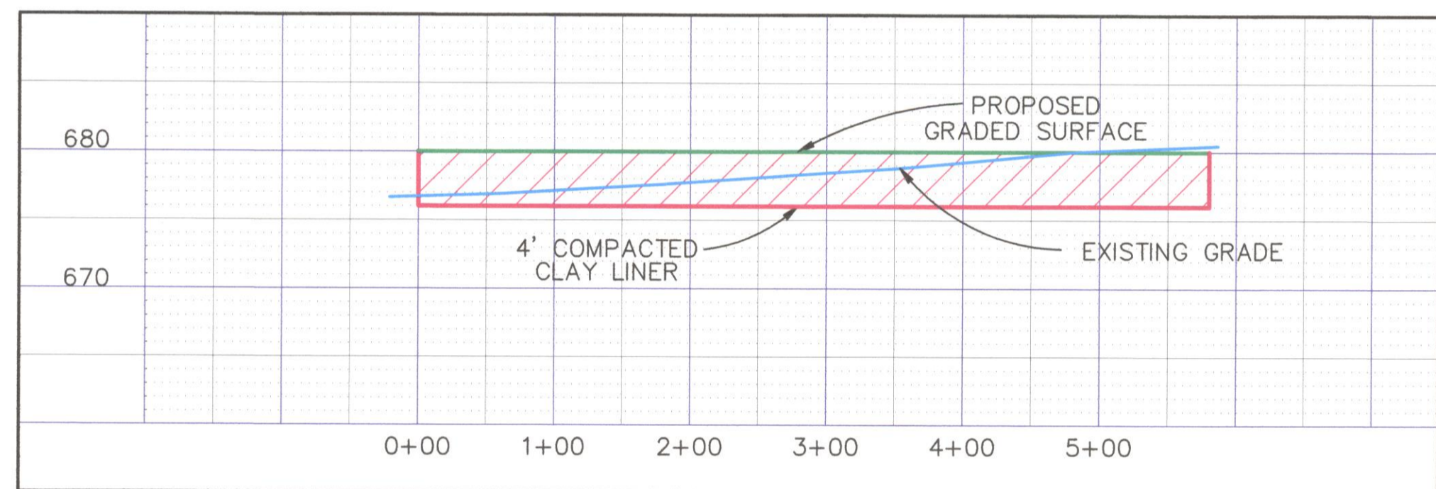
PROFILE RAW COAL AREA SCALE: 1" = 100' HORIZ. 1" = 10' VERT.
