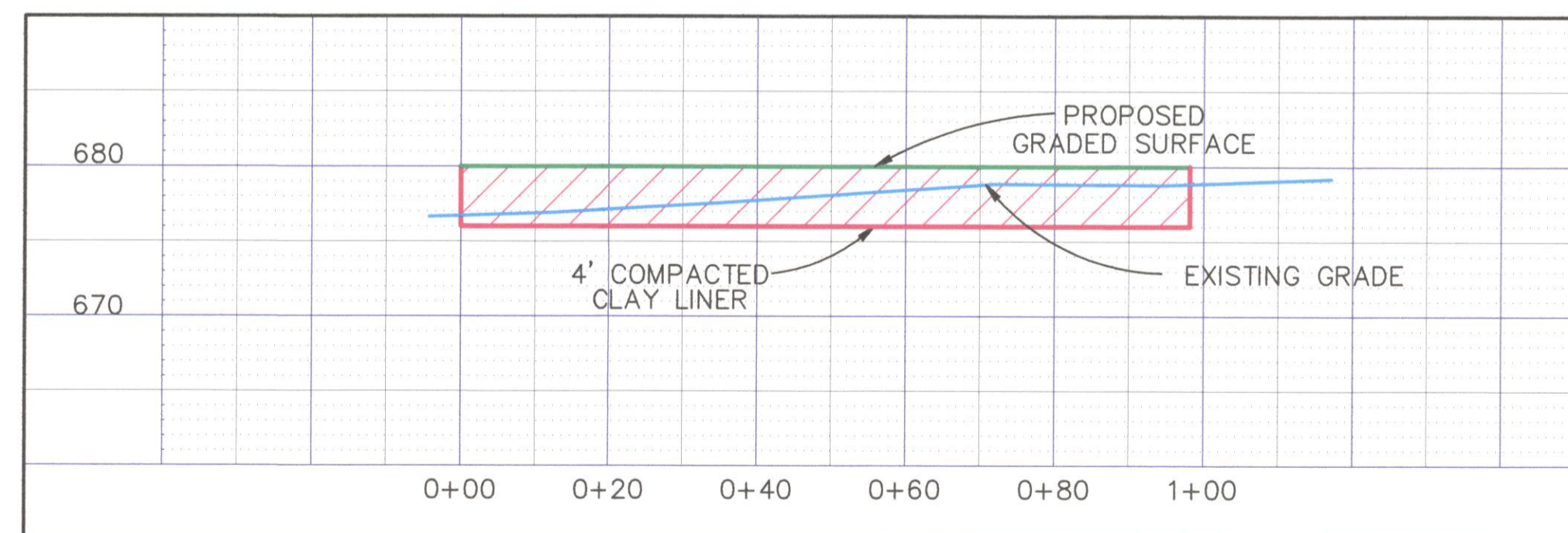
PROFILE PREP PLANT AREA SCALE: 1" = 20' HORIZ. 1" = 10' VERT.
