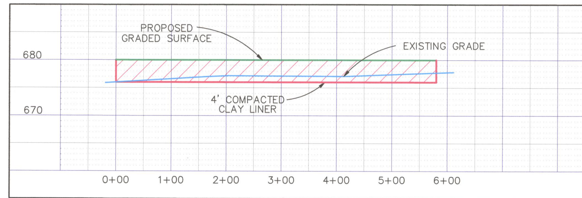
PROFILE CLEAN COAL AREA SCALE: 1" = 100' HORIZ. 1" = 10' VERT.
